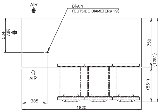
VIEW A (1/10)
